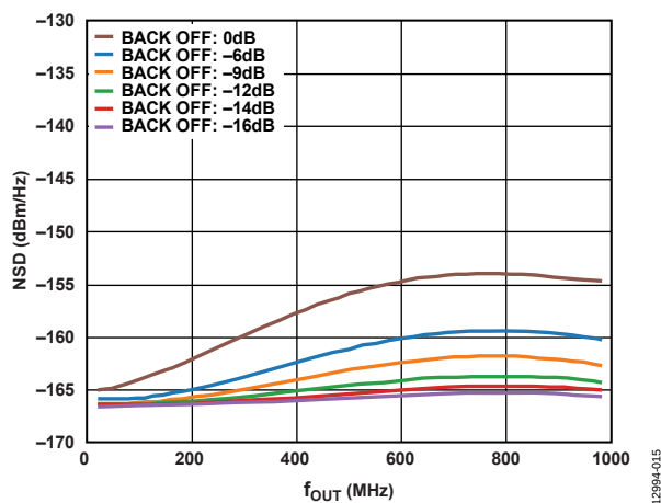
Figure 15. Single Tone NSD vs. f_{OUT} over Digital Back Off, f_{DAC} = 1966.08 MHz
