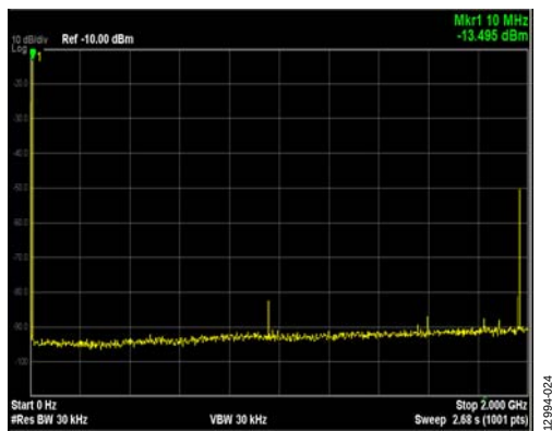
Figure 23. Two-Carrier (2C) 2x5 MHz Bandwidth with 5 MHz Gap LTE ACLR Performance, f_{DAC} = 1966.08 MHz
