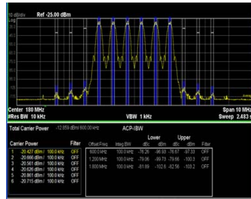
Figure 25. Six-Carrier (6C) Spaced by 600 kHz GSM Edge ACP Performance, f_{DAC} = 1966.08 MHz
