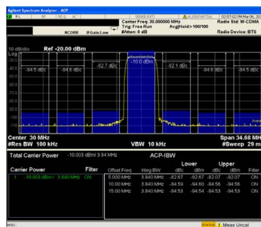
Figure 20. 1C WCDMA ACLR, f_{OUT} = 30 MHz, f_{DAC} = 983 MHz, 2 \times Interpolation, PLL Frequency = 122 MHz
