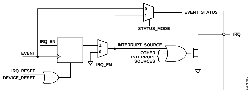
Figure 75. Simplified Schematic of \overline{\text{IRQ}} Circuitry
