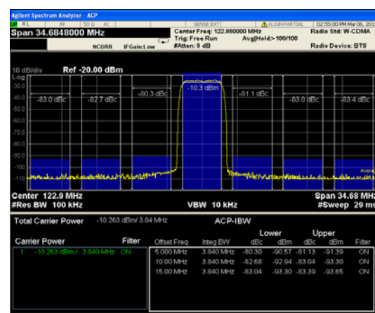
Figure 21. 1C WCDMA ACLR, f_{OUT} = 122 MHz, f_{DAC} = 983 MHz, 2 \times Interpolation, PLL Frequency = 122 MHz
