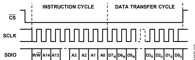
Figure 31. Serial Register Interface Timing, MSB First, ADDRINC = 0
