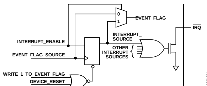
Figure 49. Simplified Schematic of \overline{IRQ} Circuitry
