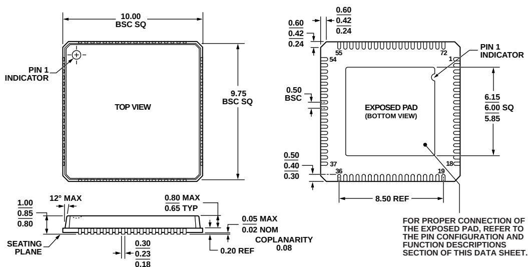
COMPLIANT TO JEDEC STANDARDS MO-220-VNND-4 Figure 89. 72-Lead Lead Frame Chip Scale Package [LFCSP_VQ] 10 mm x 10 mm Body, Very Thin Quad (CP-72-7) Dimensions shown in millimeters
