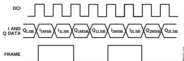
Figure 44. Timing Diagram for Byte Mode
