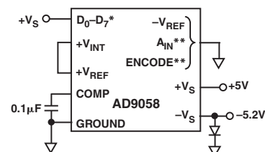
Burn-In Connections
