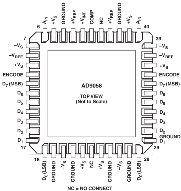
AD9058AJJ/AKJ Pinouts
