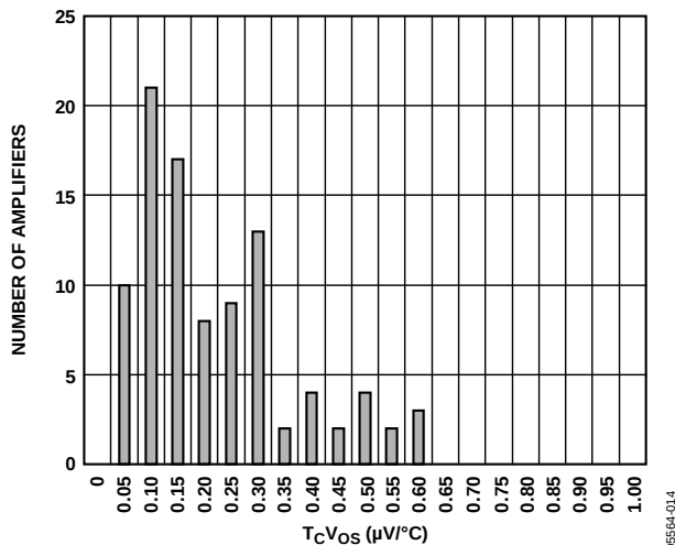
Figure 5. T_C V_{OS}
