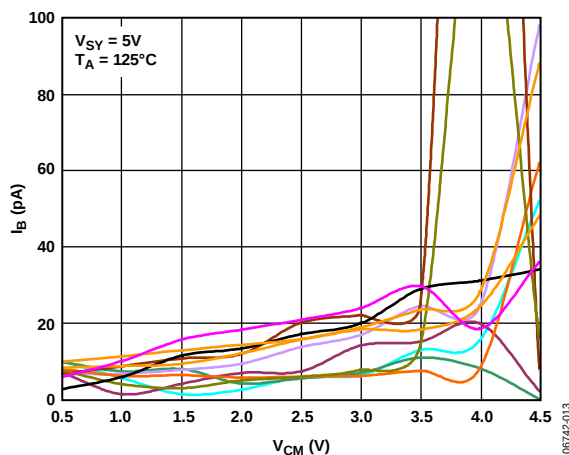
Figure 11. Input Bias Current vs. Common-Mode Voltage at 125°C
