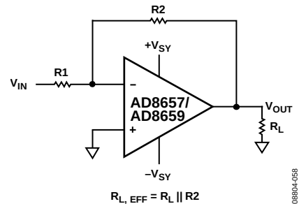
Figure 70. Inverting Op Amp Configuration
