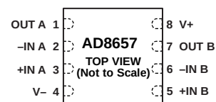
Figure 5. AD8657 Pin Configuration, 8-Lead LFCSP
