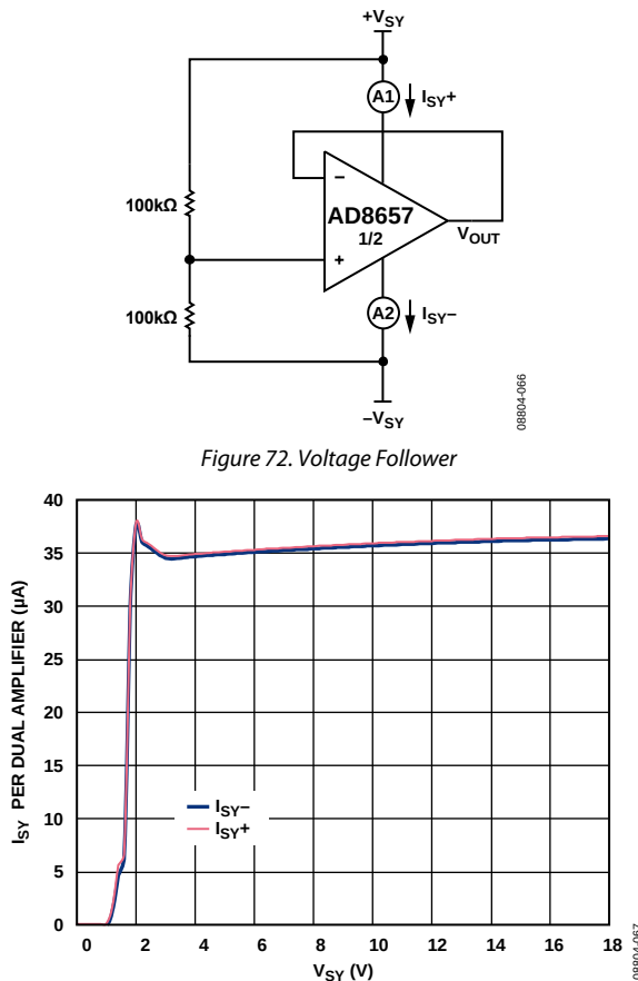
Figure 73. Supply Current vs. Supply Voltage (Voltage Follower)
