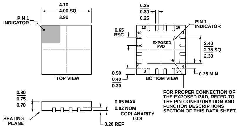
Figure 82. 16-Lead Lead Frame Chip Scale Package [LFCSP_WQ] 4 mm x 4 mm Body, Very Very Thin Quad (CP-16-20)
