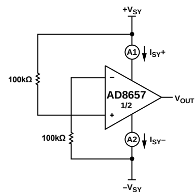
Figure 75. Comparator B
