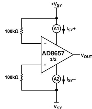
Figure 74. Comparator A
