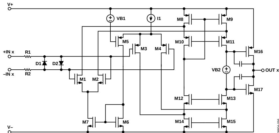
Figure 68. Simplified Schematic
