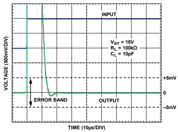
Figure 55. Positive Settling Time to 0.1%
