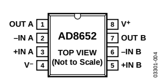
Figure 4. 8-Lead SOIC_N (R-8)
