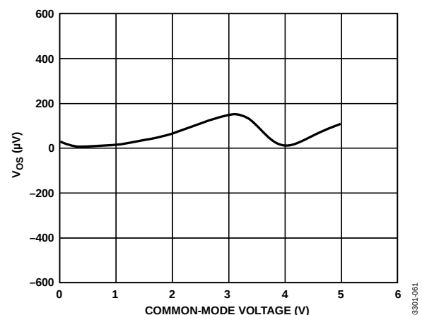
Figure 54. Input Offset Distribution over Common-Mode Voltage for the AD865x
