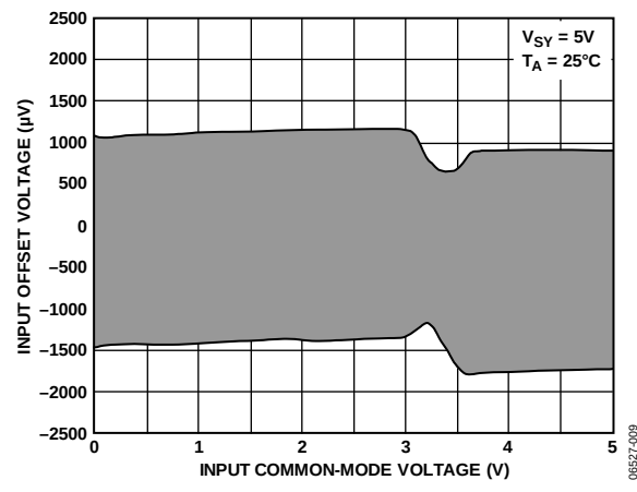
Figure 9. Input Offset Voltage vs. Input Common-Mode Voltage
