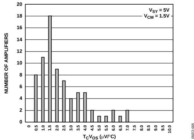
Figure 10. Offset Voltage Drift
