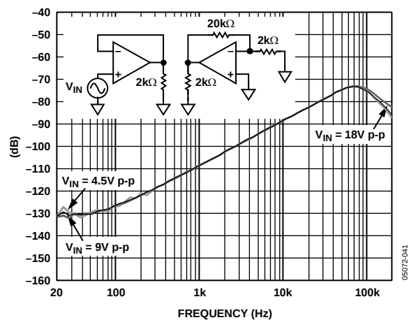
Figure 43. Channel Separation
