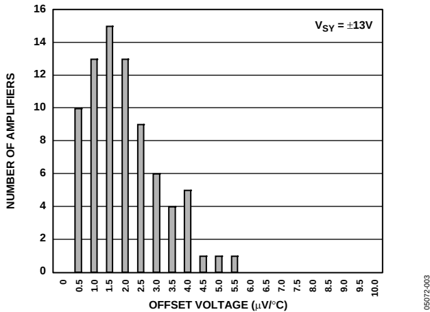
Figure 8. Offset Voltage Drift
