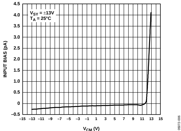
Figure 11. Input Bias Current vs. V_{CM}
