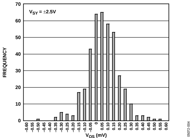
Figure 9. Input Offset Voltage
