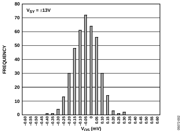
Figure 7. Input Offset Voltage
