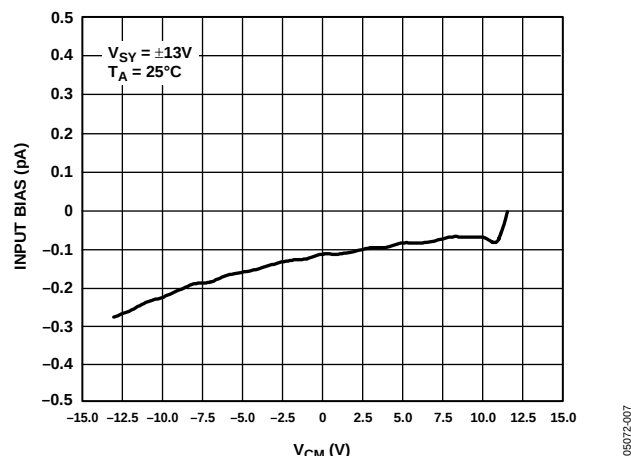
Figure 12. Input Bias Current vs. V_{CM}
