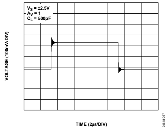
Figure 37. Driving Heavy Capacitive Loads Without Compensation
