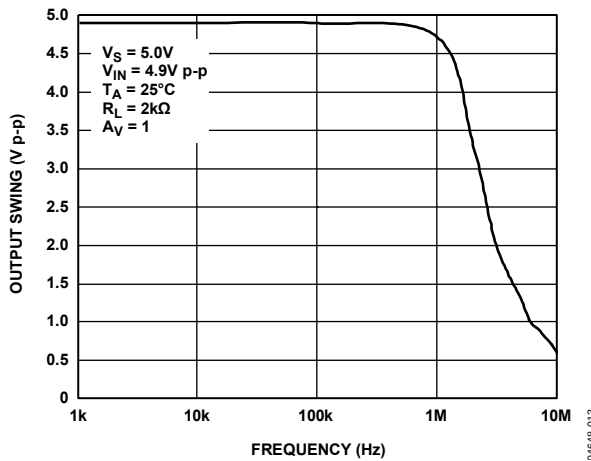
Figure 13. Closed-Loop Output Voltage Swing vs. Frequency
