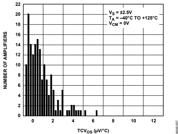
Figure 7. Offset Voltage Drift Distribution
