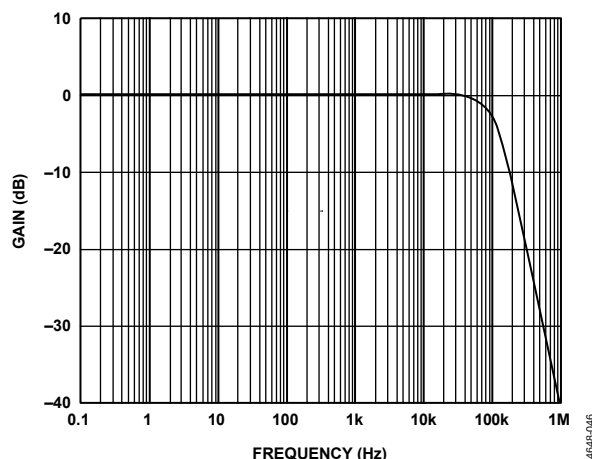
Figure 46. Second-Order Butterworth, Low-Pass Filter Frequency Response
