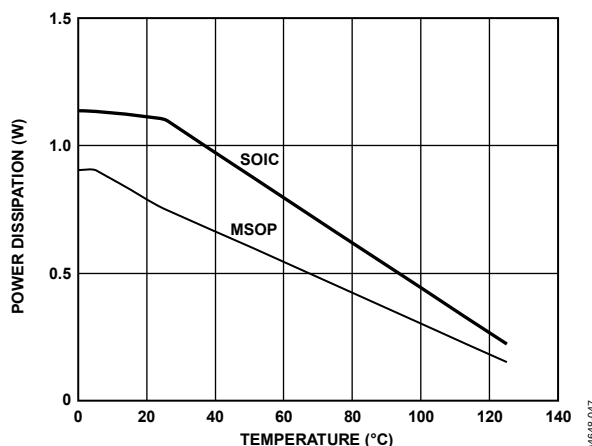
Figure 47. Maximum Power Dissipation vs. Ambient Temperature
