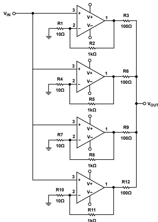
Figure 43. Noise Reduction
