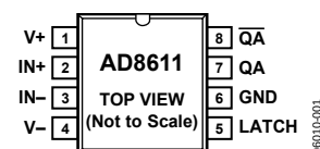
Figure 1. 8-Lead Narrow Body SOIC (R-8)
