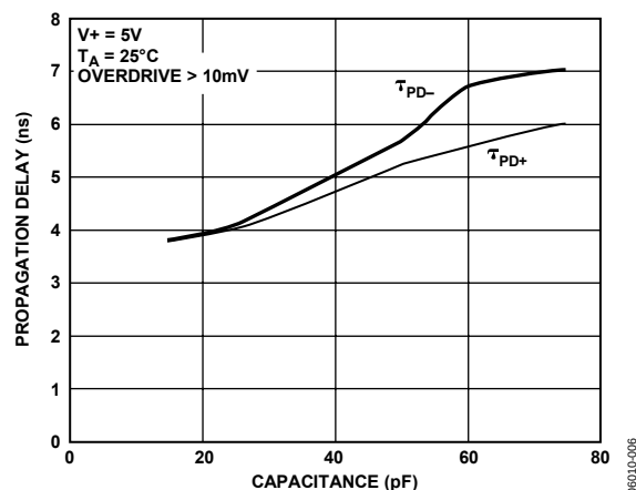
Figure 9. Propagation Delay vs. Load Capacitance
