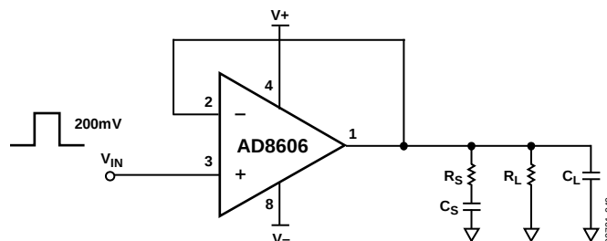
Figure 51. Snubber Network Configuration
