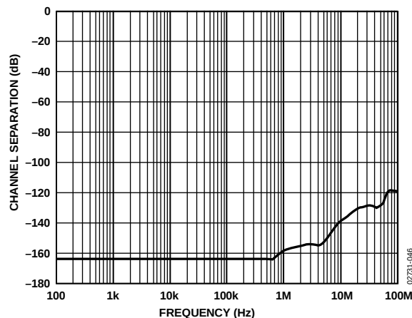
Figure 49. Channel Separation vs. Frequency
