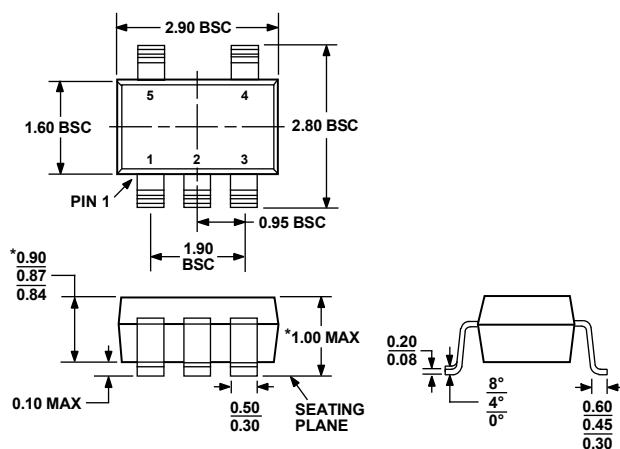
Figure 48. 5-Lead Thin Small Outline Transistor Package [TSOT] (UJ-5) Dimensions shown in millimeters
