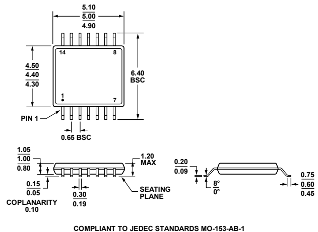
Figure 72. 14-Lead Thin Shrink Small Outline Package [TSSOP] (RU-14) Dimensions shown in millimeters
