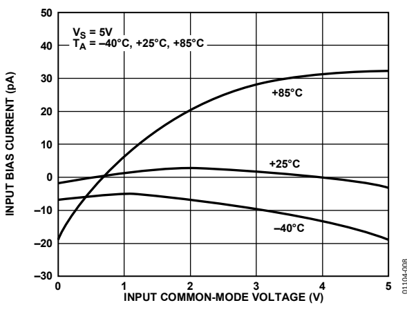
Figure 8. Input Bias Current vs. Input Common-Mode Voltage
