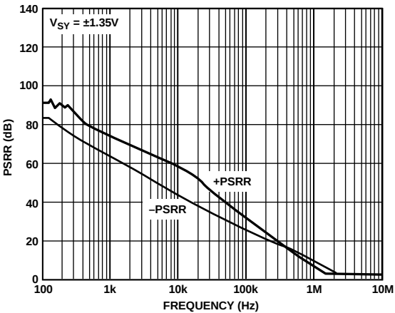
Figure 34. PSRR vs. Frequency at \pm 1.35\text{ V}
