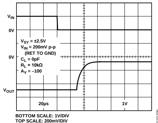
Figure 30. Negative Overvoltage Recovery
