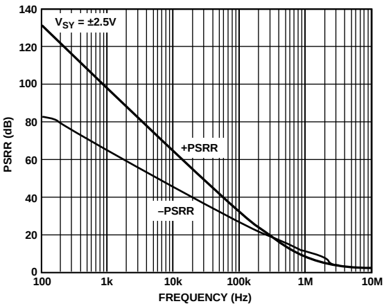
Figure 35. PSRR vs. Frequency at \pm 2.5\text{ V}
