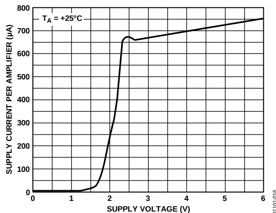
Figure 16. Supply Current per Amplifier vs. Supply Voltage
