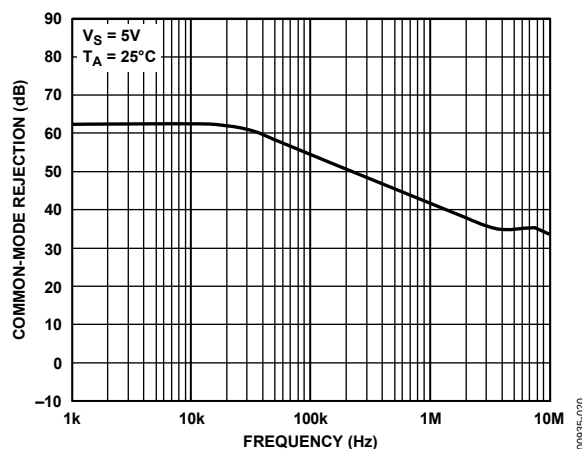
Figure 20. Common-Mode Rejection Ratio vs. Frequency
