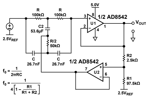
Figure 35. 60 Hz Twin-T Notch Filter, Q = 10
