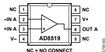
Figure 1. 8-Lead SOIC (R Suffix)
