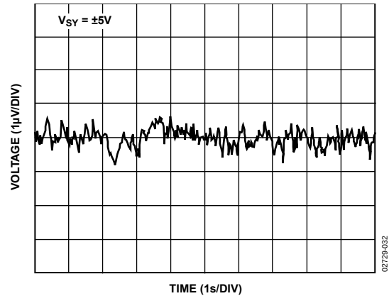
Figure 32. 0.1 Hz to 10 Hz Input Voltage Noise
