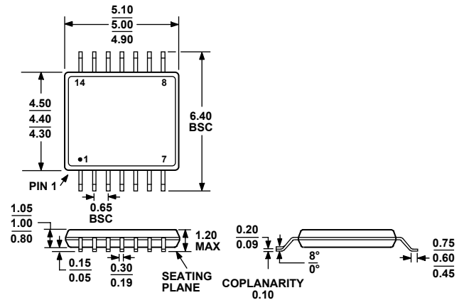
COMPLIANT TO JEDEC STANDARDS MO-153-AB-1 Figure 61. 14-Lead Thin Shrink Small Outline Package [TSSOP] (RU-14) Dimensions shown in millimeters
