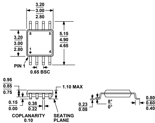
COMPLIANT TO JEDEC STANDARDS MO-187-AA Figure 60. 8-Lead Mini Small Outline Package [MSOP] (RM-8) Dimensions shown in millimeters
