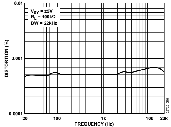
Figure 42. THD + N vs. Frequency
