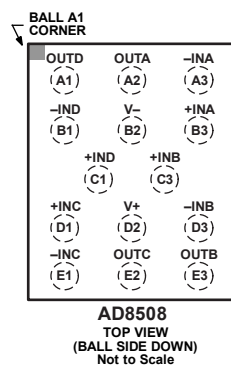
Figure 6. 14-Ball WLCSP (CB-14-1)
