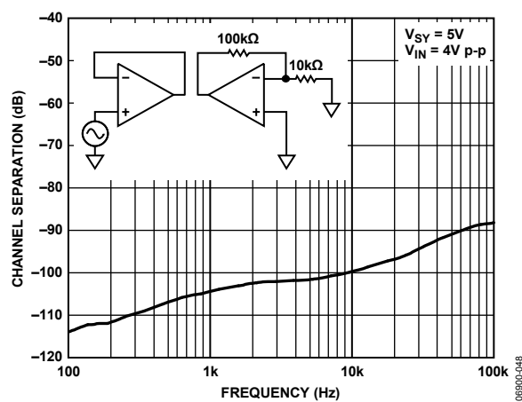
Figure 44. Channel Separation vs. Frequency
