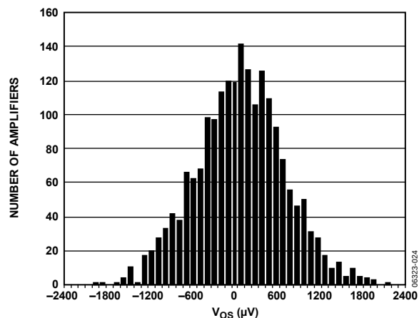
Figure 25. Input Offset Voltage Distribution ( 0\text{ V} < V_{CM} < 1.8\text{ V} ), V_S = 1.8\text{ V}
