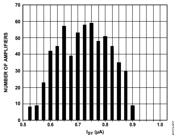
Figure 8. Supply Current Distribution, V_S = 5 V
