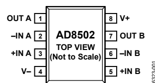
Figure 1. 8-Lead SOT-23
