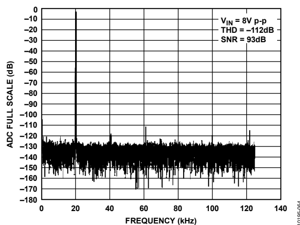
Figure 55. FFT of AD8476 Driving the AD7687
