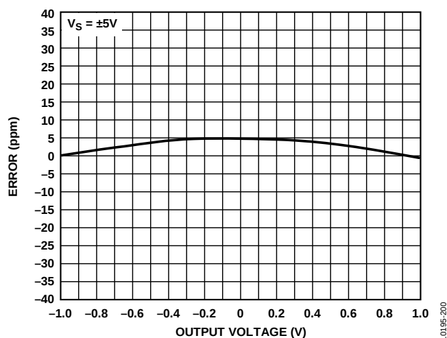
Figure 44. Gain Nonlinearity
