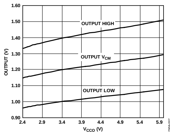
Figure 7. LVDS Output Level vs. V_{CC0}
