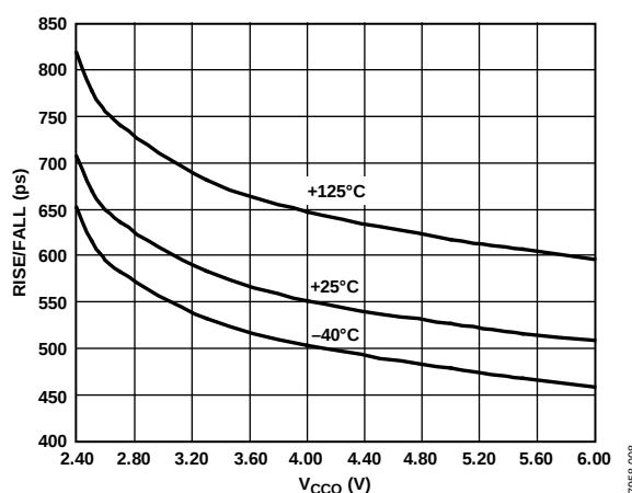
Figure 8. LVDS Output Rise/Fall Time vs. V_{CC0}
