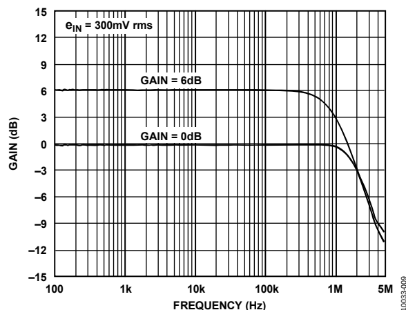
Figure 10. Input Buffer, Large Signal Bandwidth at 0 dB and 6 dB Gain
