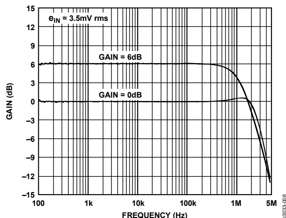
Figure 9. Input Buffer, Small Signal Bandwidth at 0 dB and 6 dB Gain
