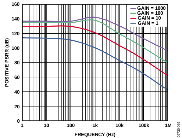
Figure 7. Positive PSRR vs. Frequency
