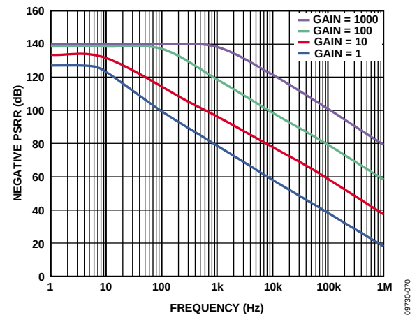
Figure 8. Negative PSRR vs. Frequency
