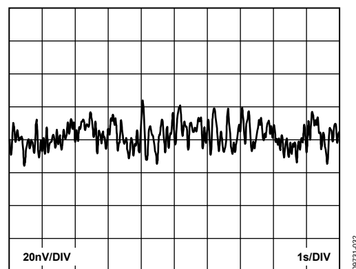
Figure 30. RTI Voltage Noise, 0.1 Hz to 10 Hz
