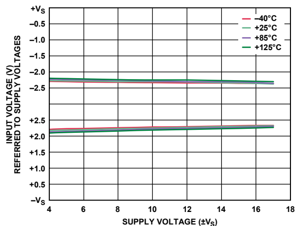
Figure 23. Input Voltage Limit vs. Supply Voltage
