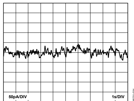
Figure 32. Current Noise, 0.1 Hz to 10 Hz
