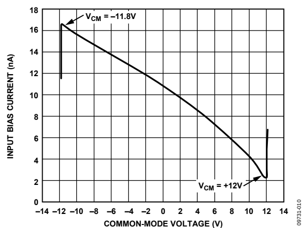
Figure 10. Input Bias Current vs. Common-Mode Voltage, V_S = \pm 15\text{ V}
