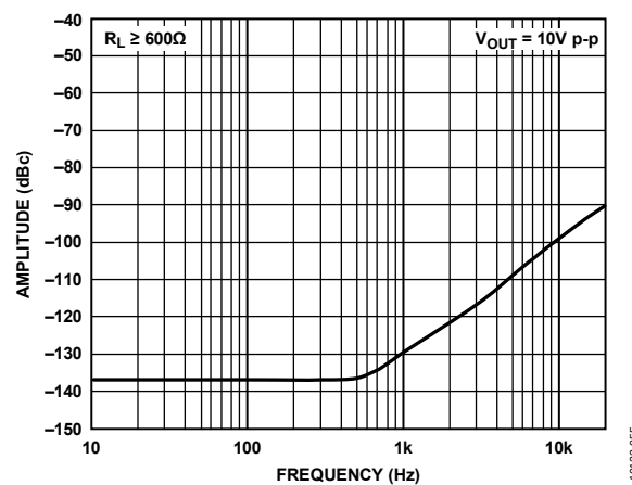
Figure 56. Second Harmonic Distortion vs. Frequency ( G = 1 )
