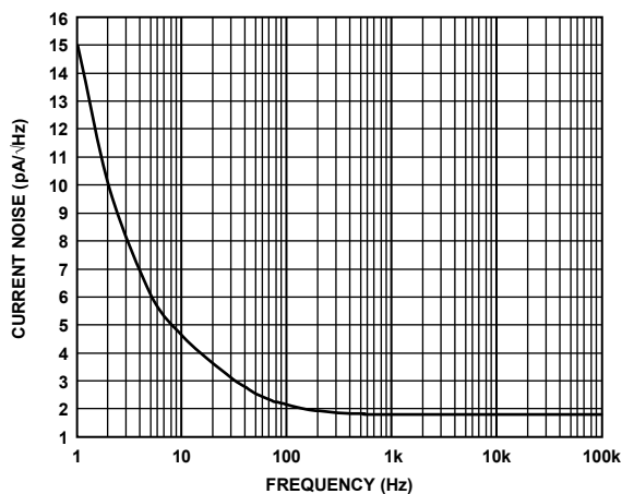
Figure 31. Current Noise Spectral Density vs. Frequency
