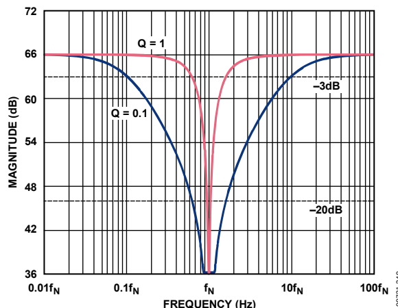
Figure 49. Notch Filter Attenuation with Q = 0.1 and Q = 1 Around the Center Frequency
