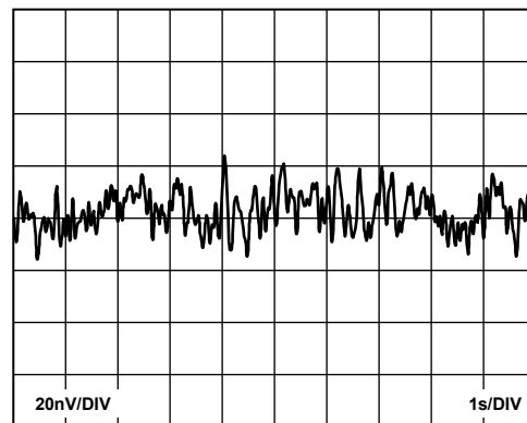
Figure 30. RTI Voltage Noise, 0.1 Hz to 10 Hz
