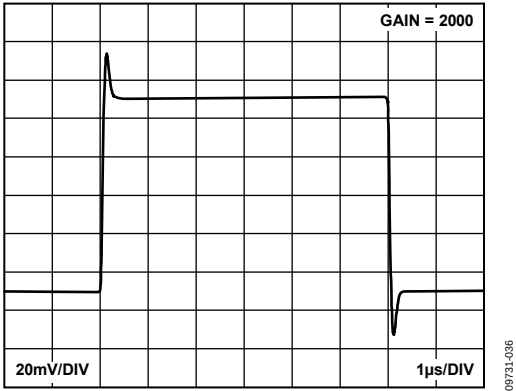
Figure 34. Small Signal Pulse Response, R_L = 10\text{ k}\Omega , C_L = 100\text{ pF}
