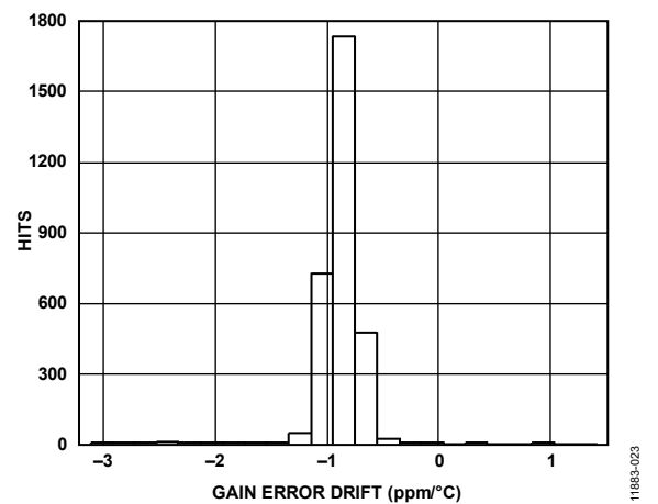
Figure 28. Gain Error Drift Distribution
