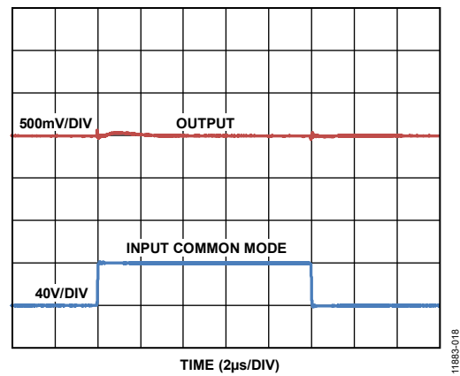
Figure 19. Input Common-Mode Step Response Large Scale ( V_S = 5V , Inputs Shorted)
