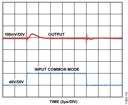
Figure 20. Input Common-Mode Step Response Small Scale ( V_S = 5V , Inputs Shorted)
