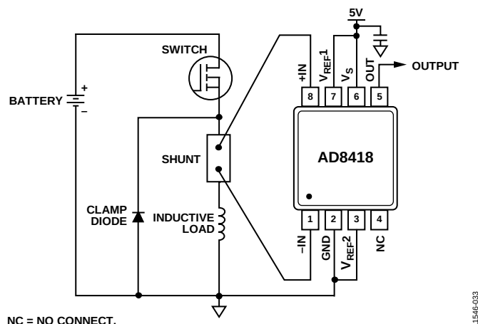
Figure 35. High-Side Switch
