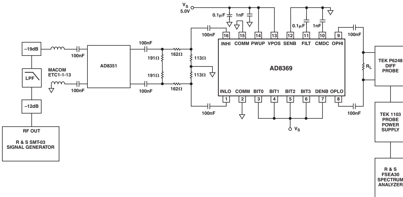
Figure 15. Harmonic Distortion Setup
