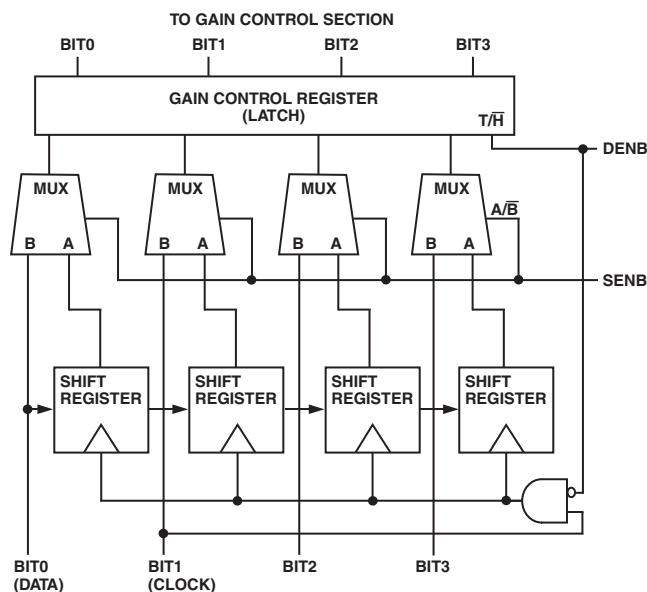
Figure 2. Digital Interface Block Diagram
