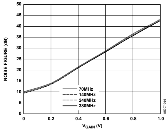
Figure 16. Noise Figure vs. V_{GAIN} ( V_{MODE} = 0\text{ V} )
