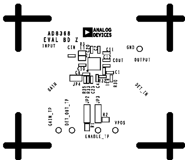
Figure 41. Component Side Silkscreen
