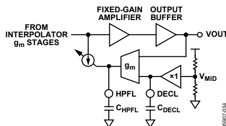
Figure 31. Output Centering Control Loop
