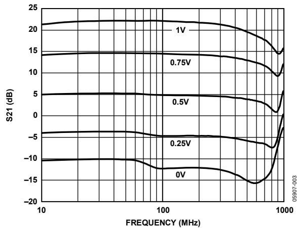
Figure 3. S21 vs. Frequency by V_{\text{GAIN}}
