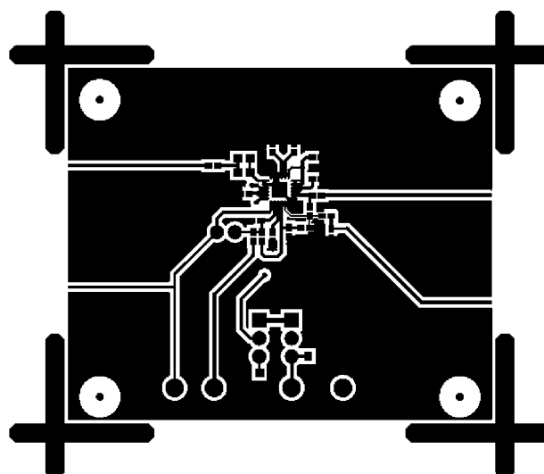
Figure 43. Component Side Layout
