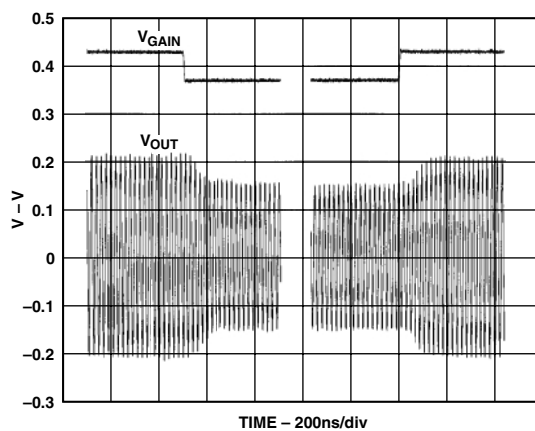
TPC 17. VGA Time Domain Response (3 dB Step)
