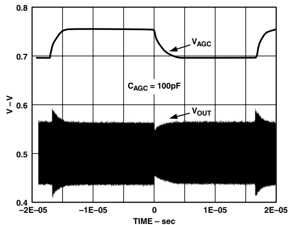
TPC 22. AGC Time Domain Response (3 dB Step)
