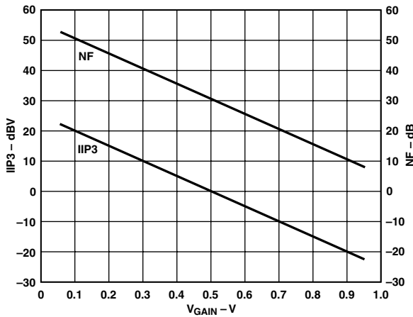
Figure 4. Noise Figure and Input Third Order Intercept vs. Gain ( R_{\text{SOURCE}} = 200 \Omega )
