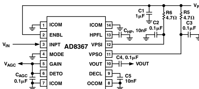
Figure 8. Basic Connections for AGC Operation
