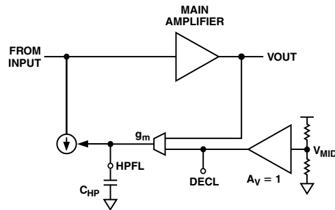
Figure 5. The dc output level is centered to mid supply by a control loop whose corner frequency is determined by C_{\text{HP}} .
