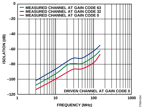
Figure 37. Channel-to-Channel Isolation vs. Frequency, Channel A Driven, Channel B Measured
