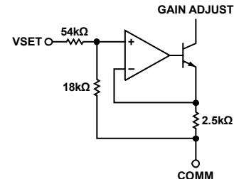
Figure 40. VSET Interface Simplified Schematic
