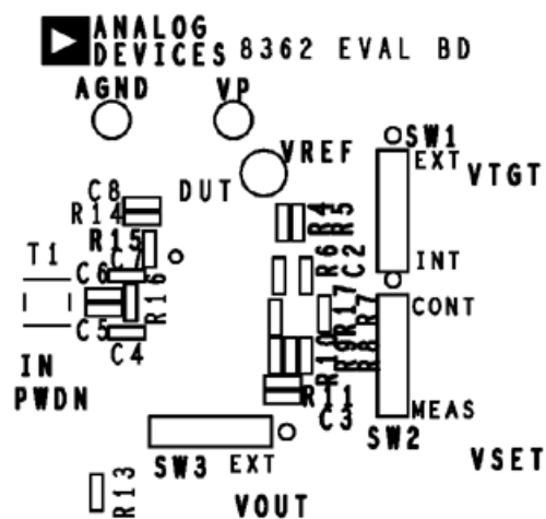
Figure 68. Component Side Metal of Evaluation Board
