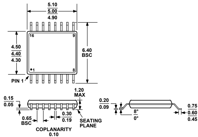
Figure 70. 16-Lead Thin Shrink Small Outline Package [TSSOP] (RU-16) Dimensions shown in millimeters
