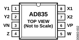
Figure 2. Pin Configuration
