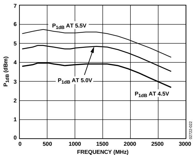
Figure 23. P_{1\text{dB}} vs. Frequency, V_S = 4.5\text{ V} , 5\text{ V} , and 5.5\text{ V} , T_A = 25^\circ\text{C}
