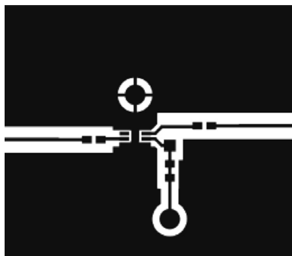
Figure 43. Component Side
