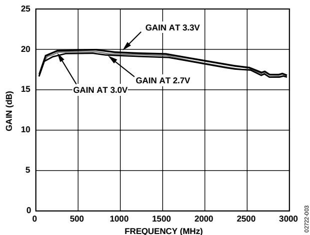
Figure 4. Gain vs. Frequency, V_S = 2.7\text{ V} , 3\text{ V} , and 3.3\text{ V} , T_A = 25^\circ\text{C}
