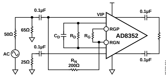
Figure 26. Single-Ended Schematic
