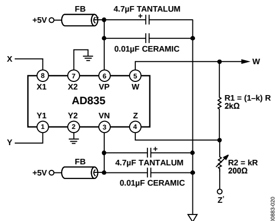
Figure 20. Multiplier Connections
