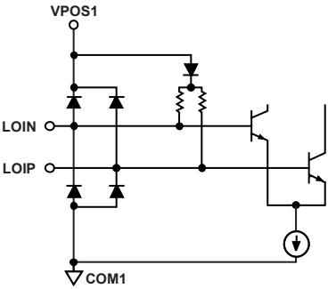
Figure 3. Circuit A
