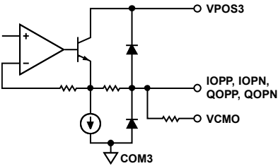
Figure 4. Circuit B
