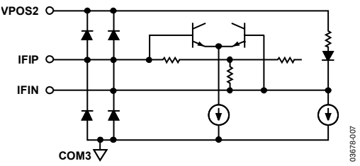
Figure 7. Circuit E
