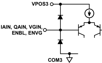
Figure 6. Circuit D
