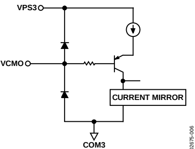
Figure 38. Circuit C
