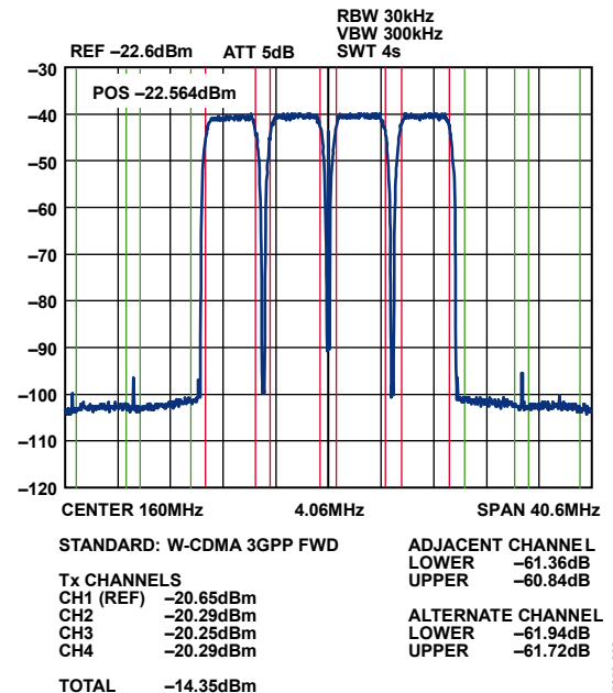
Figure 55. ACPR Performance for Multiple W-CDMA Carriers Being Downconverted from 2140 MHz to 160 MHz for Distortion Analysis
