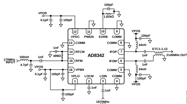
Figure 51. W-CDMA Tx Upconversion Application Circuit
