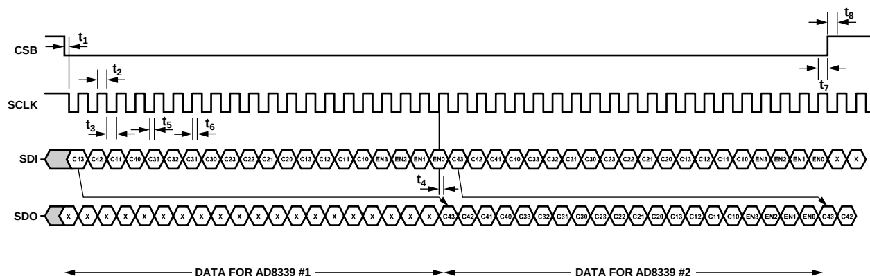
Figure 57. Timing Diagram
