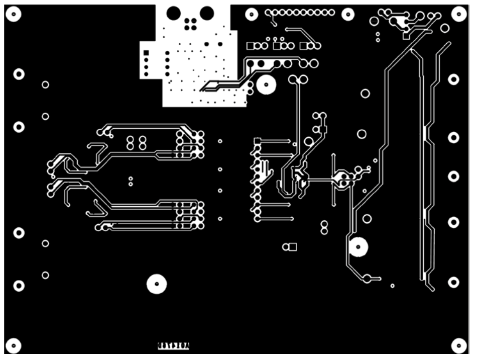
Figure 67. AD8339-EVALZ Wiring Side Copper
