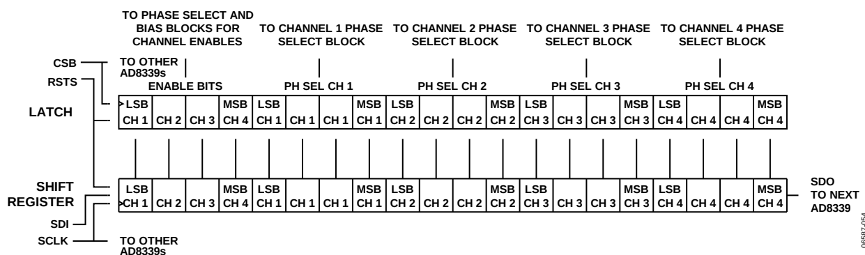
Figure 56. Serial Interface Showing the 20-Bit Shift Register and Latch
