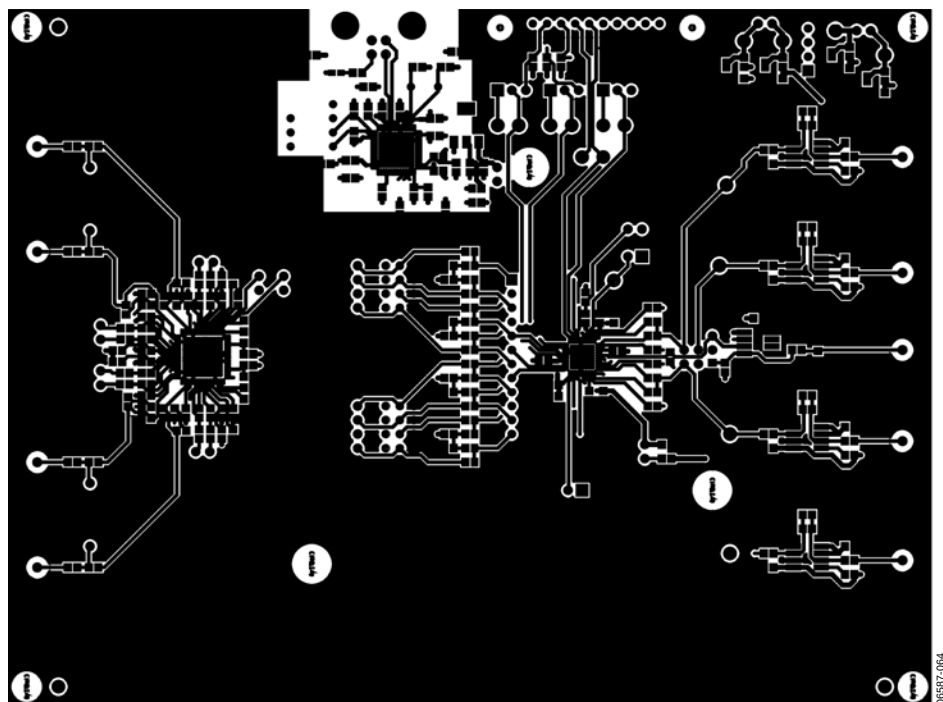
Figure 66. AD8339-EVALZ Component Side Copper
