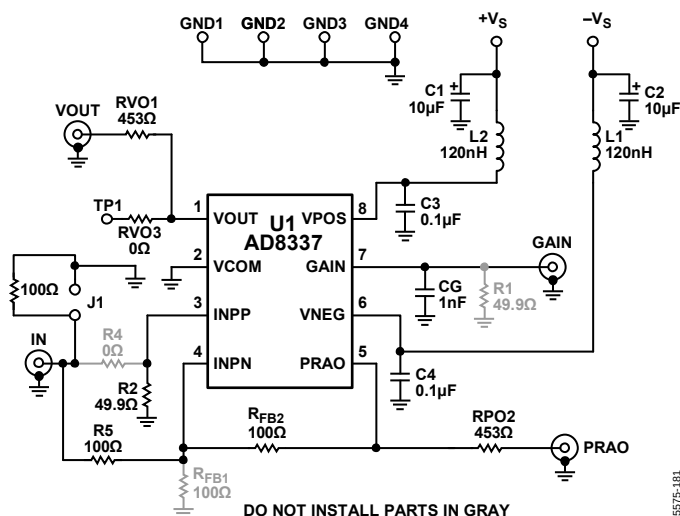
Figure 81. Schematic—AD8337-EVALZ-INV Inverting Configuration
