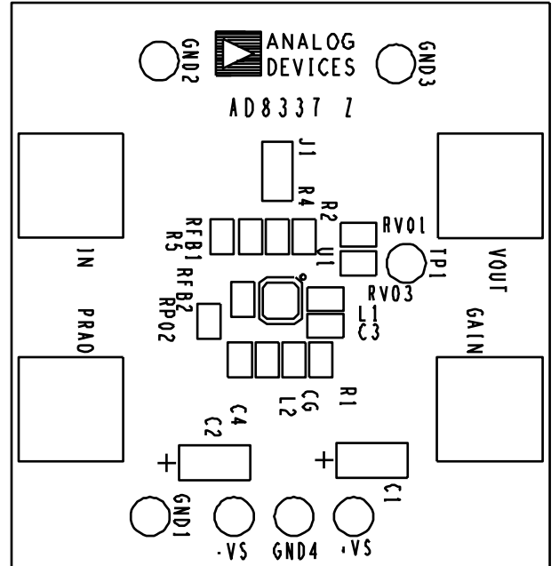
Figure 78. Assembly, Dual-Supply Evaluation Board
