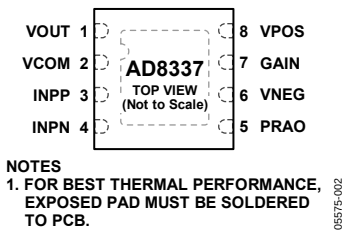
Figure 2. Pin Configuration
