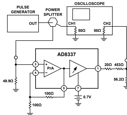
Figure 53. Pulse Response
