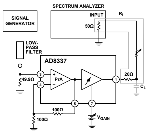
Figure 52. Harmonic Distortion
