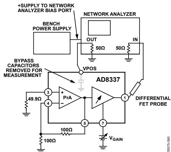
Figure 60. PSRR
