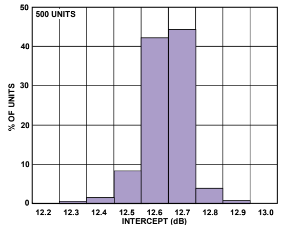
Figure 8. Intercept Histogram
