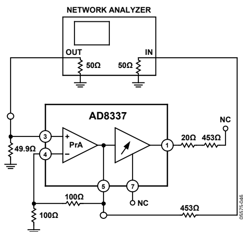
Figure 46. Frequency Response—Preamplifier
