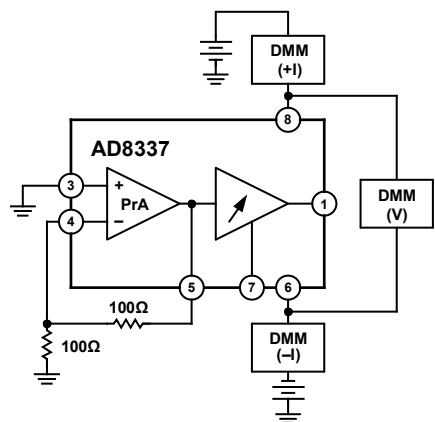
Figure 57. Supply Current
