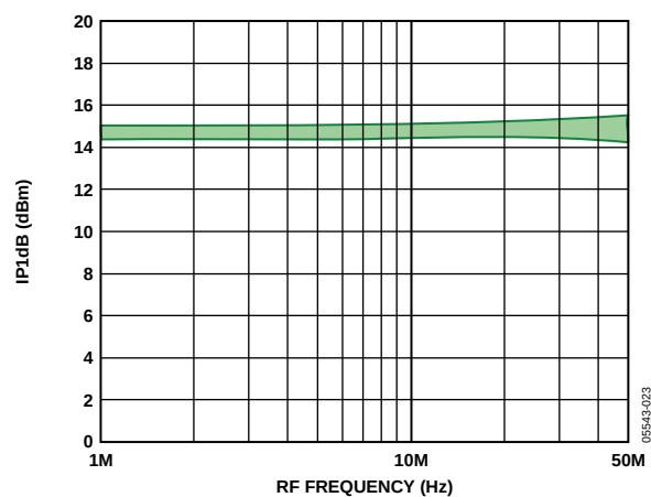
Figure 24. IP1dB vs. RF Frequency, Baseband Frequency = 10 kHz, First Quadrant (see Figure 42)
