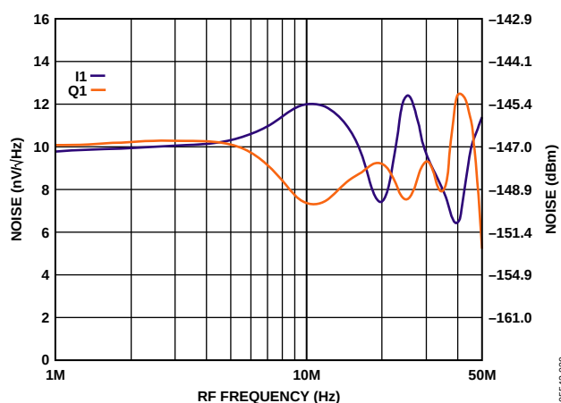
Figure 30. Input-Referred Noise vs. RF Frequency
