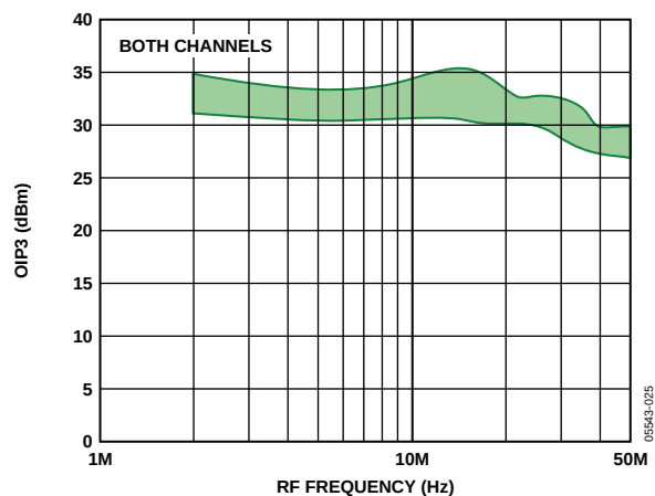
Figure 26. Representative Range of OIP3 vs. RF Frequency, First Quadrant (see Figure 49)
