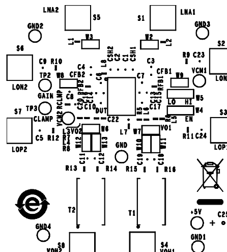
Figure 9. Component Side Silkscreen
