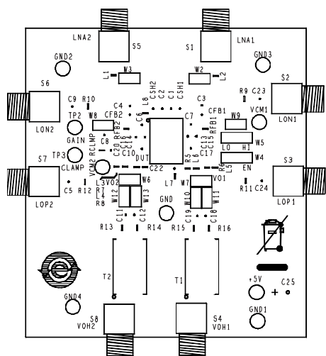
Figure 4. AD8332-EVALZ Assembly
