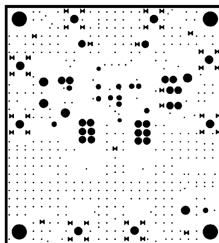
Figure 7. Ground Plane
